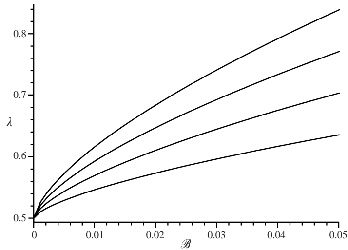
FIGURE 8. Sketch of \lambda vs. \mathcal{B} dependence for the MS boundary conditions (Vanden-Broeck 1983).
