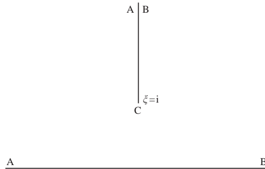
FIGURE 7. Upper half- \xi -plane, with a cut on the imaginary axis from \xi = i to i\infty .
